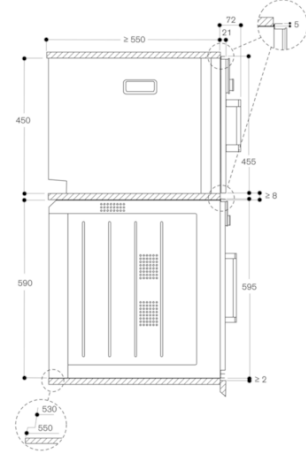
Side view of BSP 220/250 above BOP
