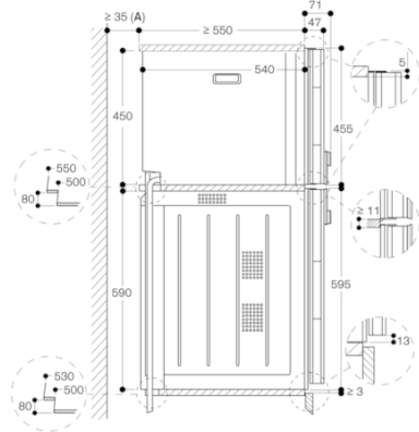
Side view of BS 474/475 above B0
